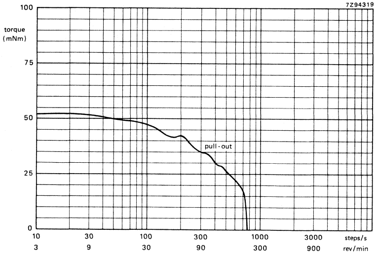
Fig. 3 Typical curve if the pull-out torque versus stepping rate measured at room temperature in the circuit of Fig. 2.
