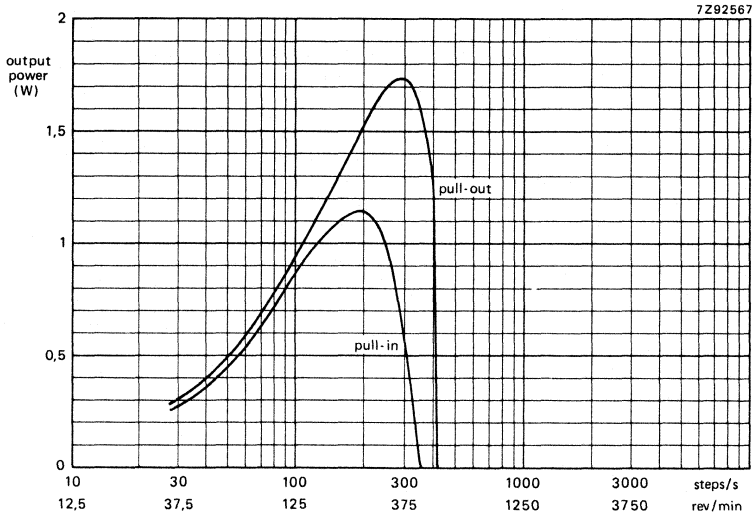
Fig. 5 Output power versus stepping rate, measured at room temperature. (type 9904 112 35116)
