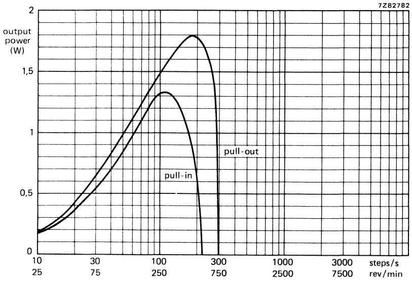
Fig. 5 Output power versus stepping rate measured at room temperature. (type 9904 112 34101)
