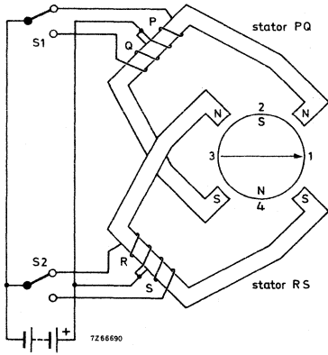
Fig. 1a. Two stator motors (4-phase).
