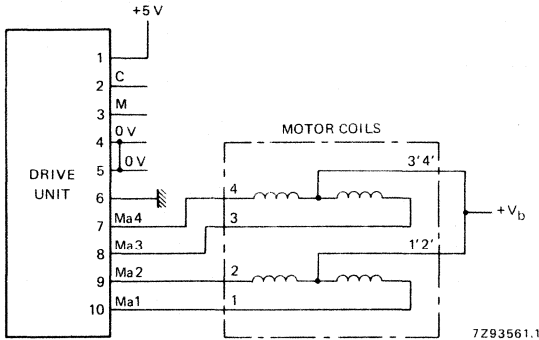
Fig. 2 Unipolar drive circuit 9904 131 03006, V_b = 12 V.
