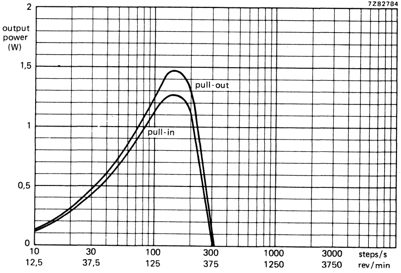
Fig. 5 Output power versus stepping rate measured at room temperature. (type 9904 112 33104)
