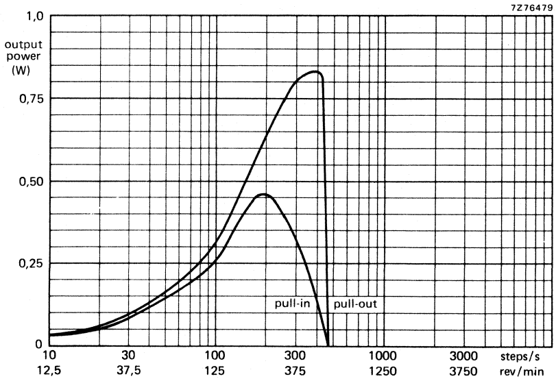
Fig. 5 Output power versus stepping rate, measured at room temperature. (type 9904 112 31101)
