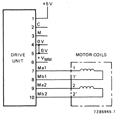
Fig. 2 Bipolar constant current drive circuit 9904 131 03007, V_{mm} = 24 V.
