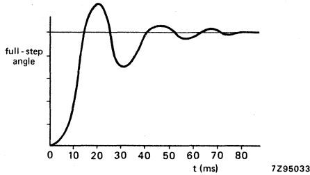
Fig. 10 Single-step response.
