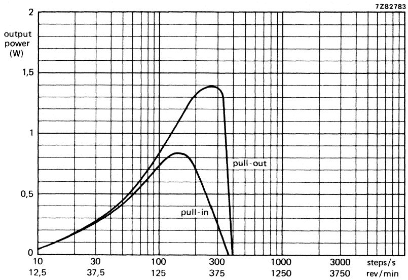
Fig. 5 Output power versus stepping rate, measured at room temperature. (type 9904 112 35114)
