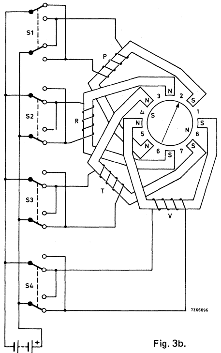
Fig. 3 Four stator motors (4-phase).
