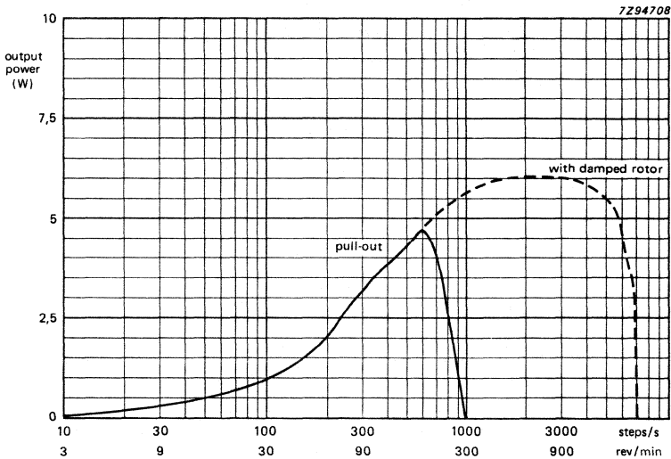
Fig. 6 Output power versus stepping rate, measured at room temperature.
