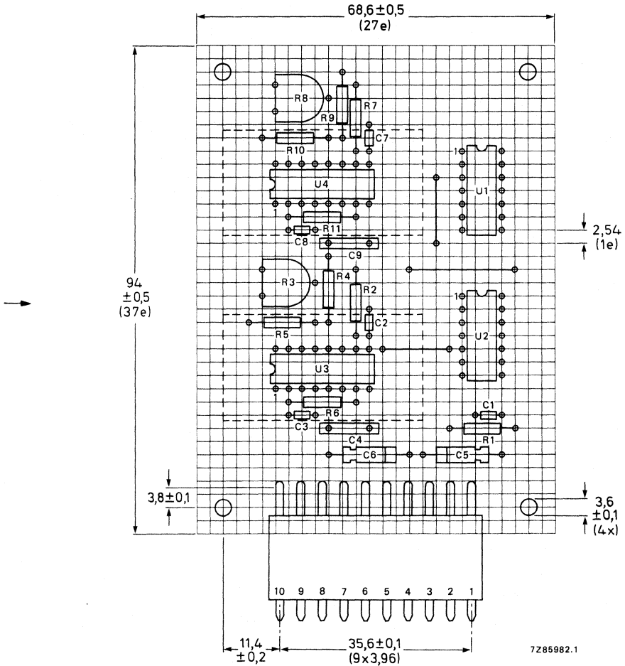
Fig. 1 Board thickness: 1,6 mm; Cu thickness: 35 µm; tracks cover with solderresist, class 1.
