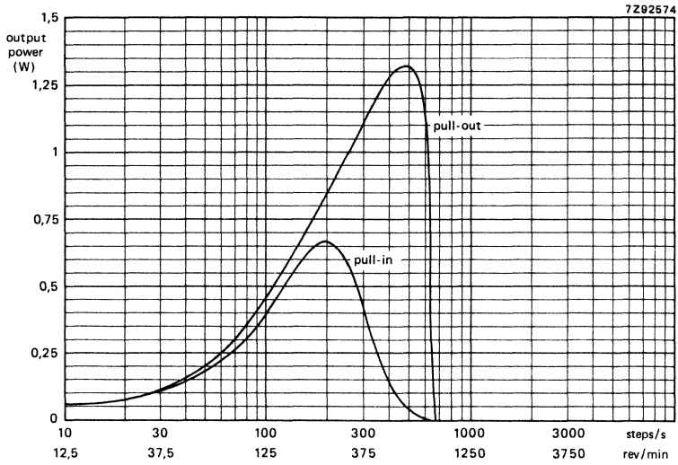
Fig. 5 Output power versus stepping rate, measured at room temperature. (type 9904 112 31106)
